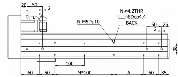
Mechanical View 5
