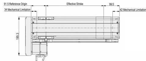
Mechanical View 1
