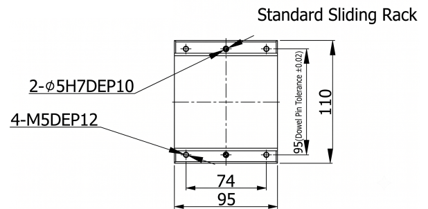
Mechanical View 2
