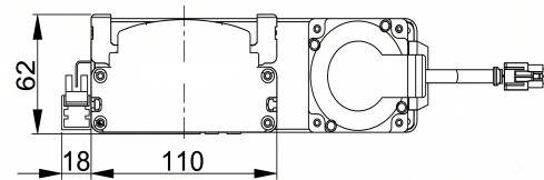
Mechanical View 4
