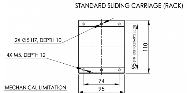
Mechanical View 2
