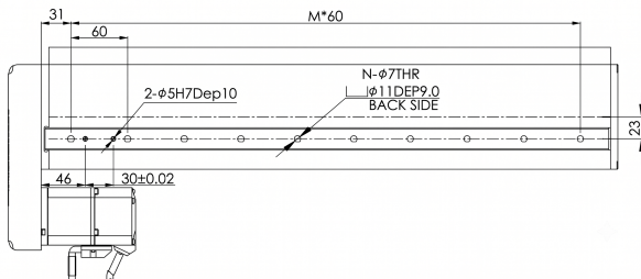
Mechanical View 5
