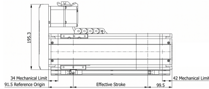
Mechanical View 1
