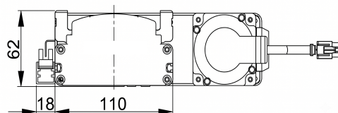
Mechanical View 4
