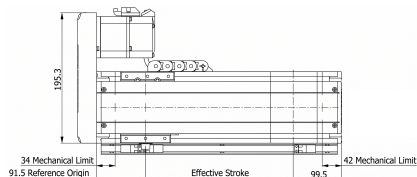
Mechanical View 1
