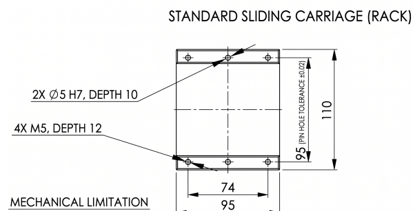
Mechanical View 2
