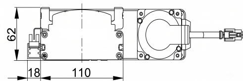
Mechanical View 4
