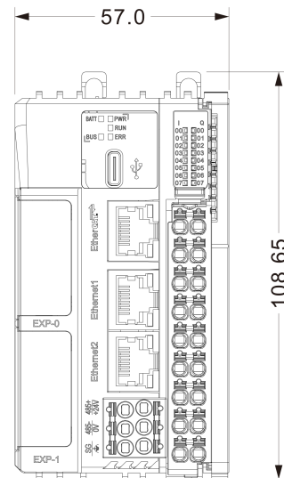
Mechanical View 4
