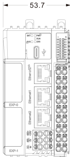
Mechanical View 1
