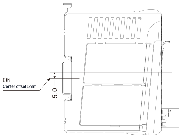
Mechanical View 3
