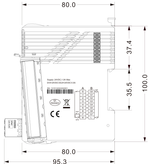
Mechanical View 2
