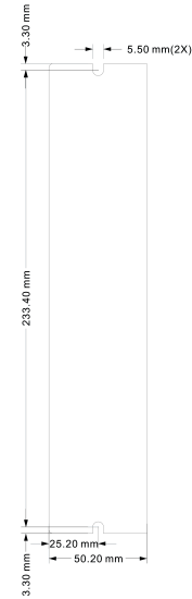
Mechanical View 2
