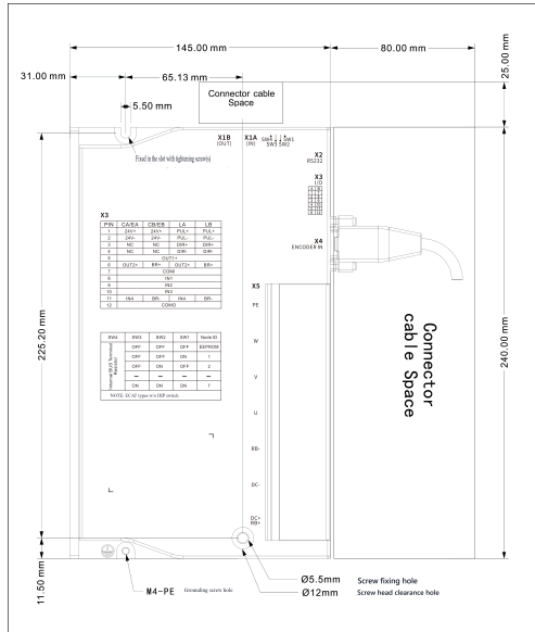
Mechanical View 1
