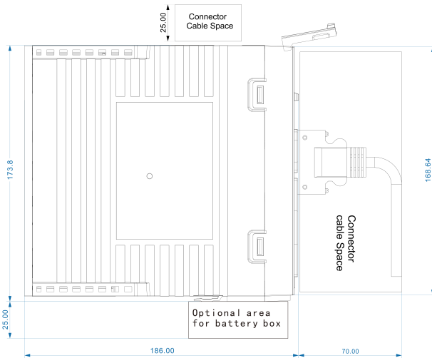
Mechanical View 1
