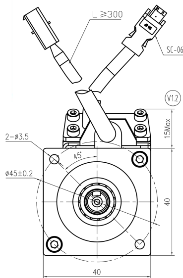
Mechanical View 6
