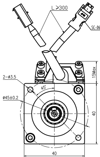
Mechanical View 5
