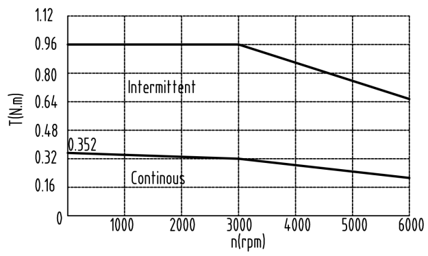
Mechanical View 8
