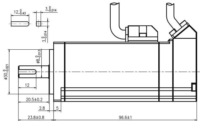
Mechanical View 7
