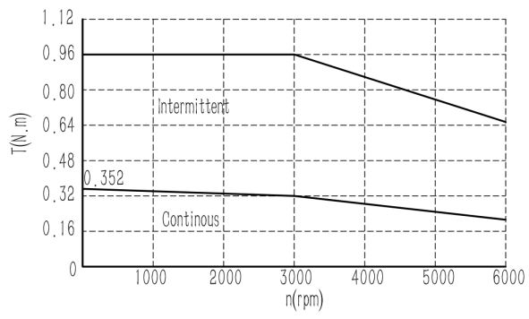
Mechanical View 8
