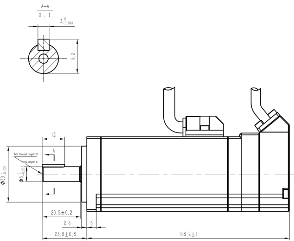
Mechanical View 5
