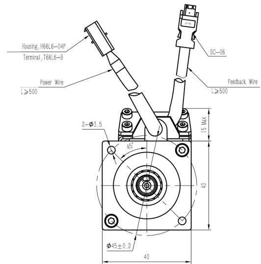
Mechanical View 6
