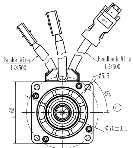
Mechanical View 8
