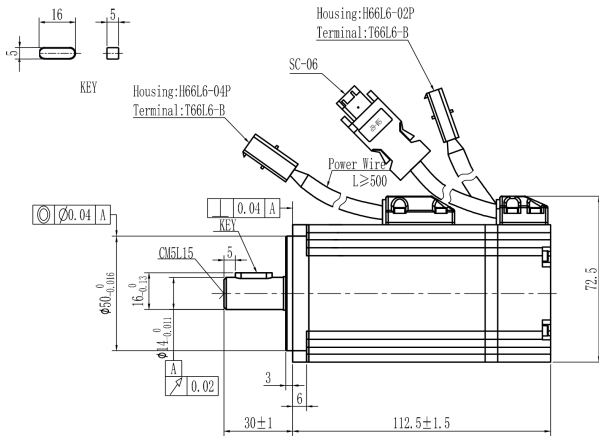
Mechanical View 6
