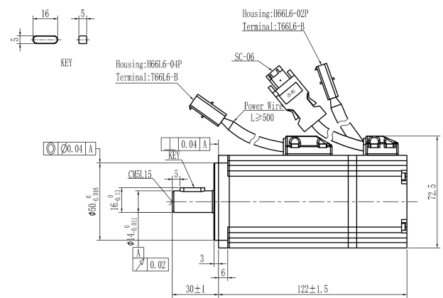
Mechanical View 7
