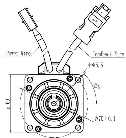
Mechanical View 6
