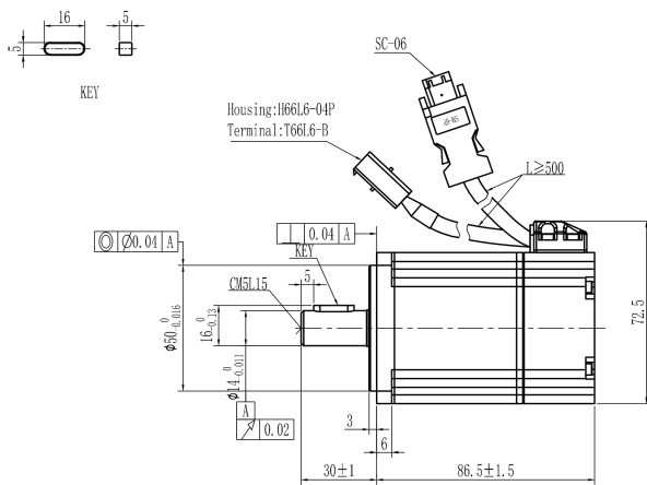
Mechanical View 5
