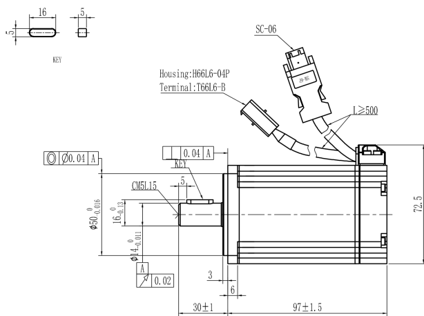
Mechanical View 5
