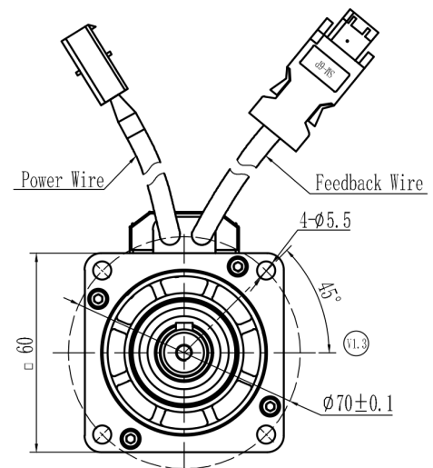
Mechanical View 6
