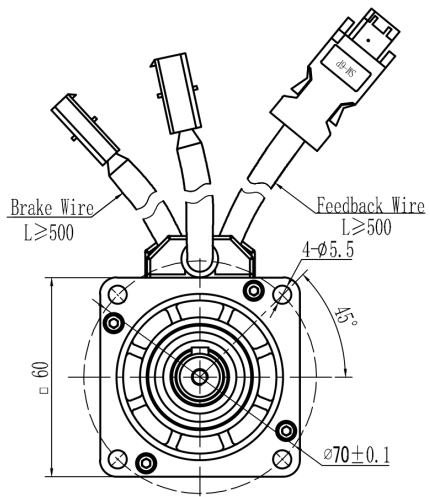
Mechanical View 8
