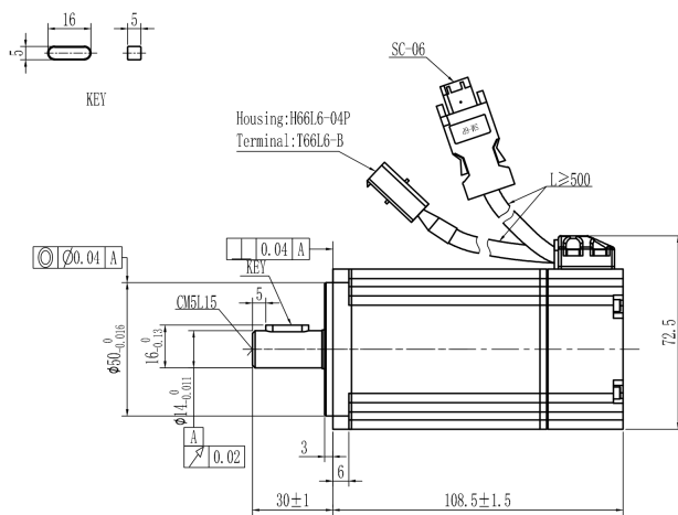
Mechanical View 7
