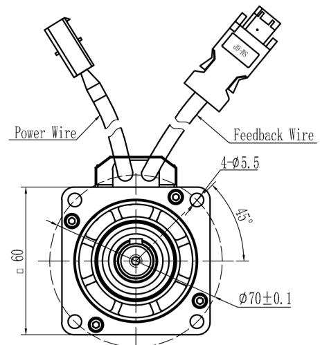
Mechanical View 8
