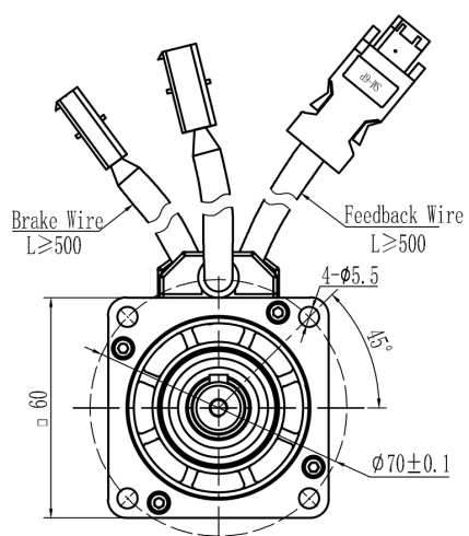
Mechanical View 8
