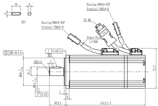
Mechanical View 7
