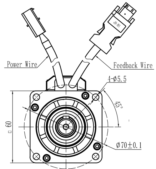
Mechanical View 6
