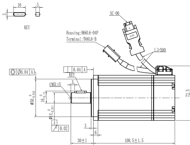
Mechanical View 5
