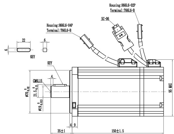
Mechanical View 7
