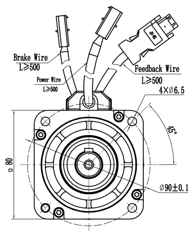
Mechanical View 8
