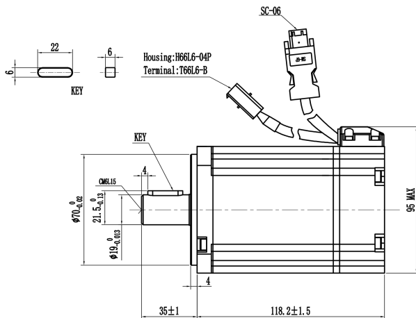
Mechanical View 5
