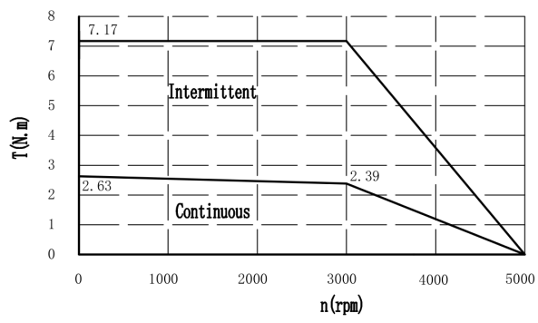
Performance Curve
