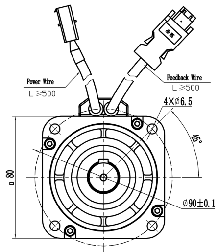
Mechanical View 6
