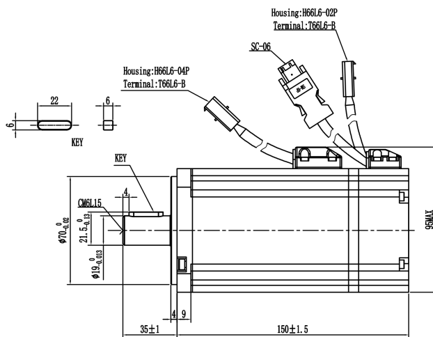
Mechanical View 7
