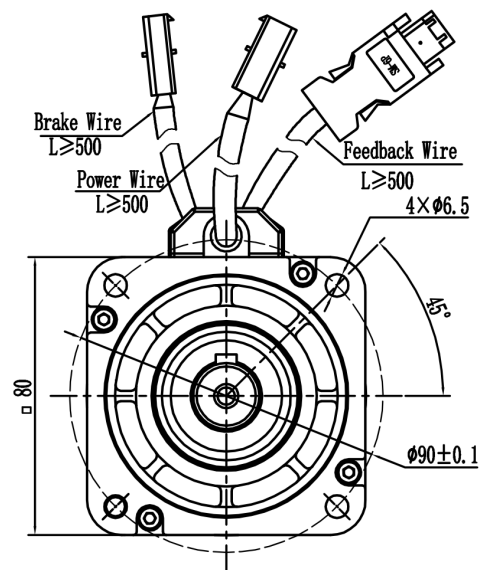
Mechanical View 9
