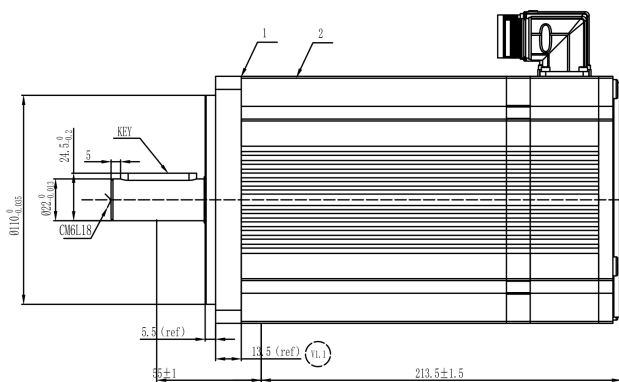
Mechanical View 6
