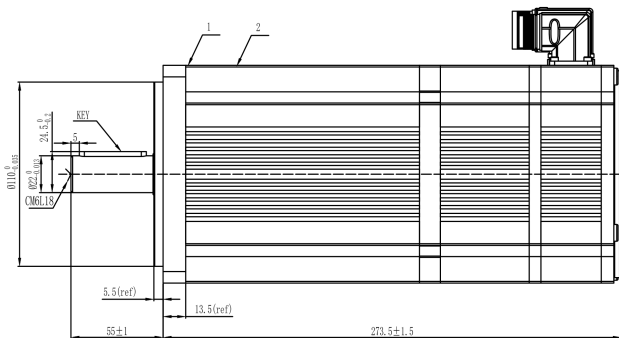
Mechanical View 7
