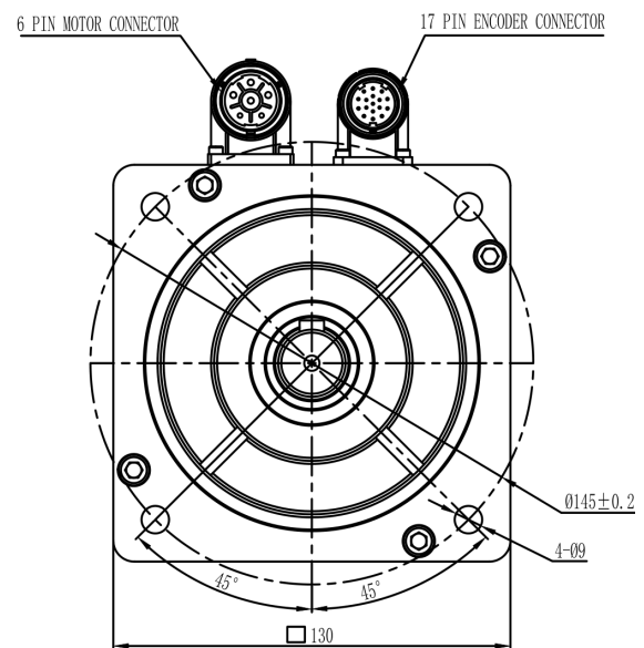
Mechanical View 7
