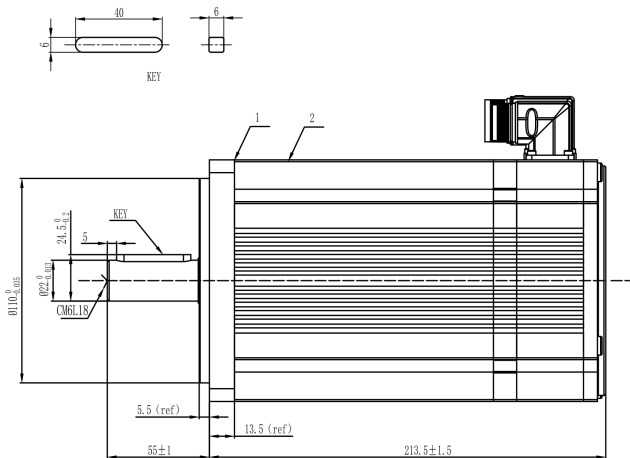
Mechanical View 6
