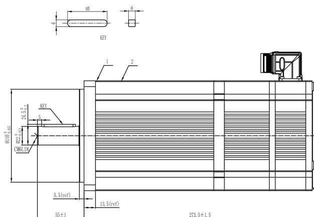
Mechanical View 7
