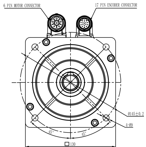
Mechanical View 8
