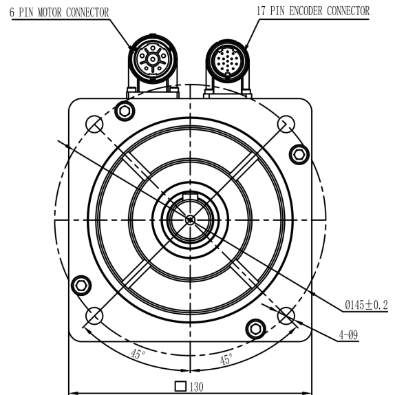
Mechanical View 7
