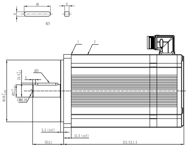
Mechanical View 6
