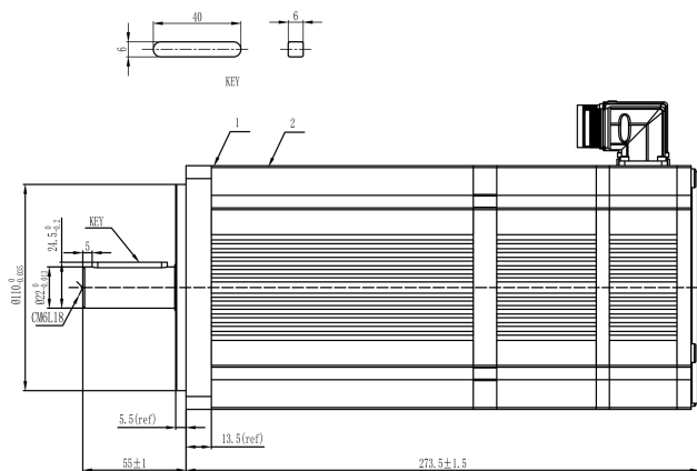
Mechanical View 7
