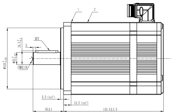
Mechanical View 6
