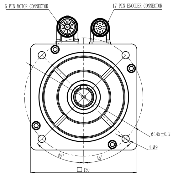
Mechanical View 7
