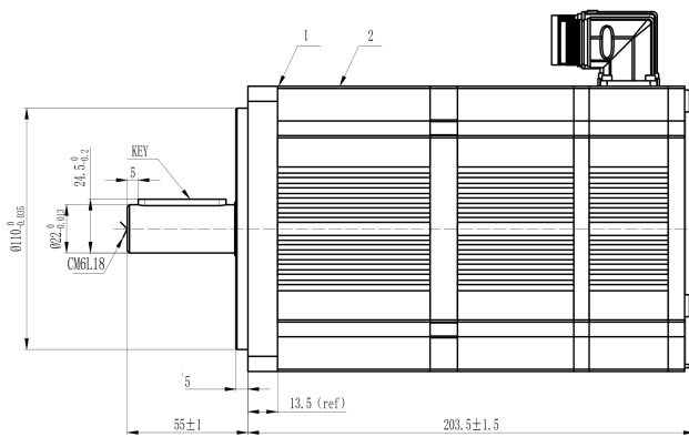
Mechanical View 6
