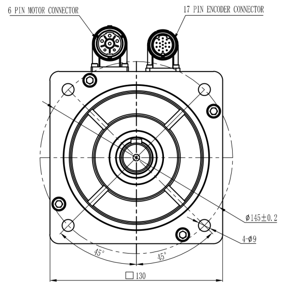
Mechanical View 8
