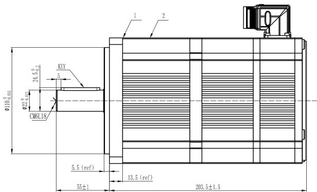
Mechanical View 7
