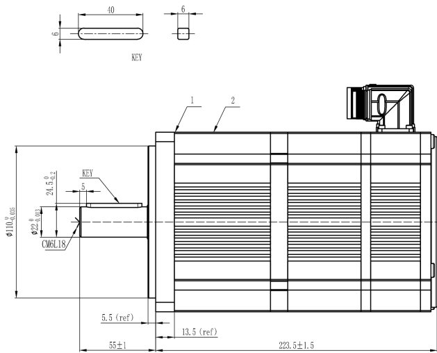
Mechanical View 7
