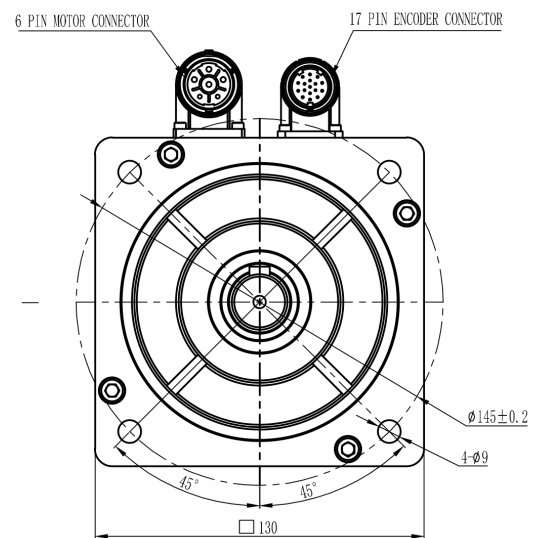
Mechanical View 8
