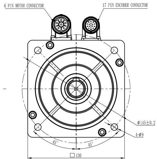
Mechanical View 7
