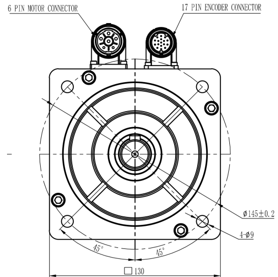
Mechanical View 7
