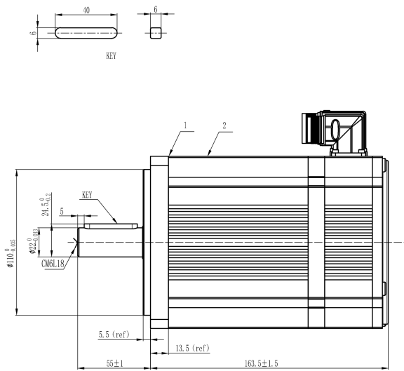
Mechanical View 6
