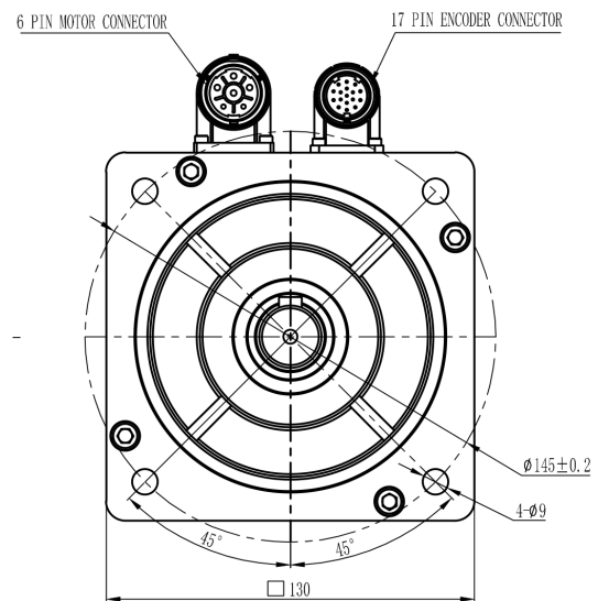
Mechanical View 8
