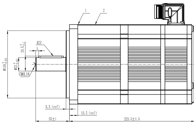
Mechanical View 7
