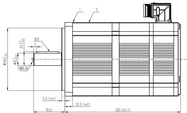
Mechanical View 8
