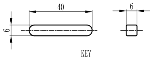
Mechanical View 6
