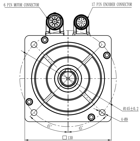
Mechanical View 7
