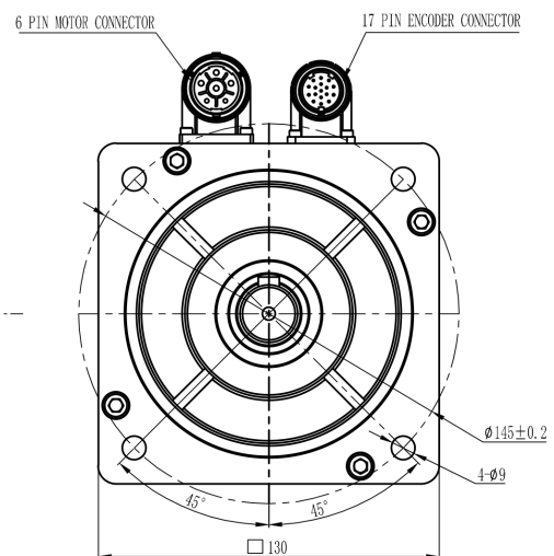
Mechanical View 7
