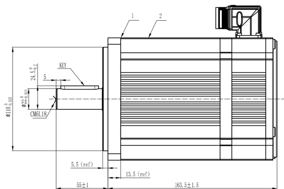
Mechanical View 6
