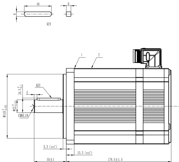
Mechanical View 6
