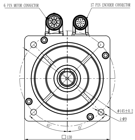
Mechanical View 8
