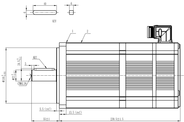
Mechanical View 7
