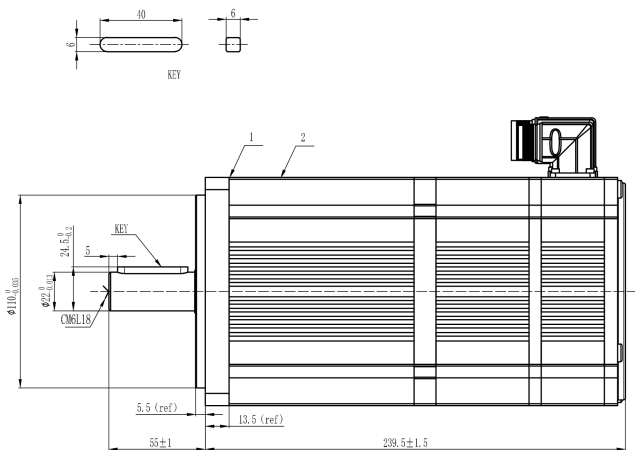
Mechanical View 7
