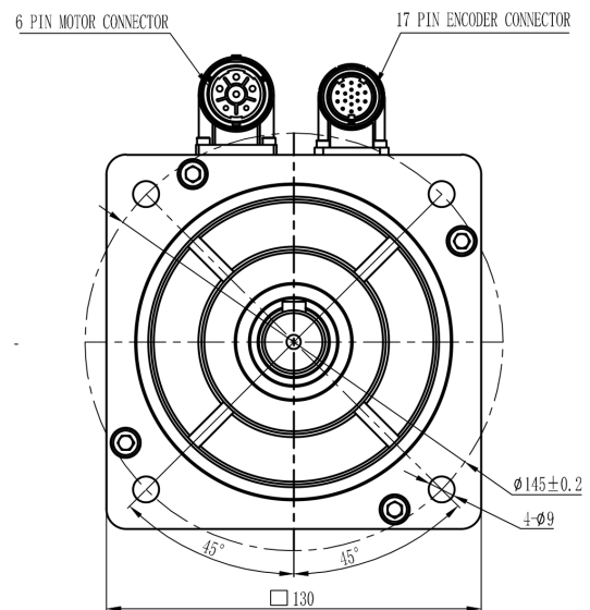
Mechanical View 8
