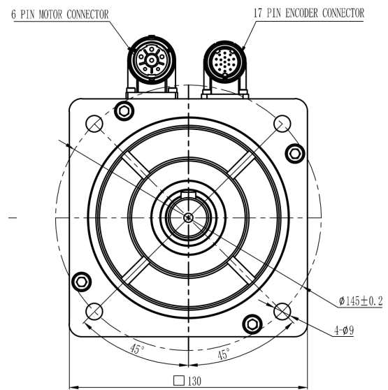
Mechanical View 7
