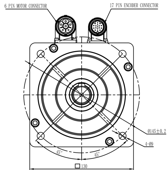
Mechanical View 6
