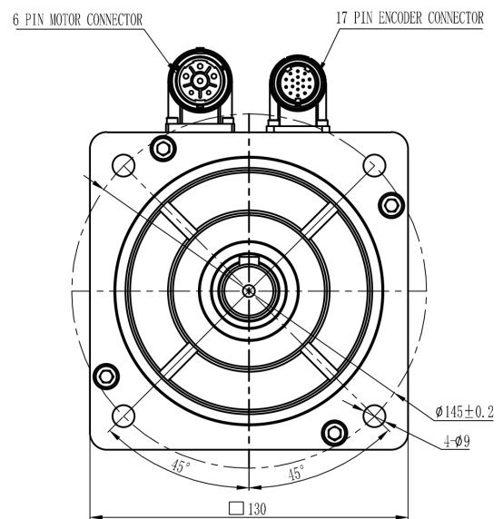
Mechanical View 7
