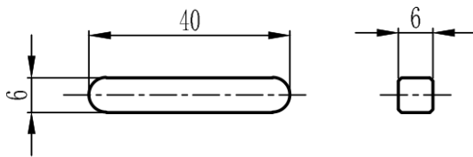
Mechanical View 6
