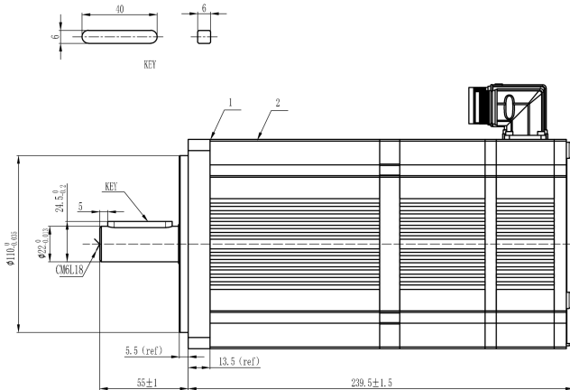
Mechanical View 7
