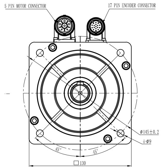
Mechanical View 8
