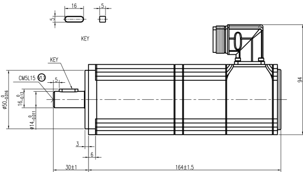
Mechanical View 7
