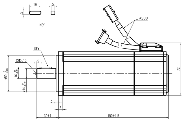
Mechanical View 7
