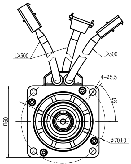
Mechanical View 10
