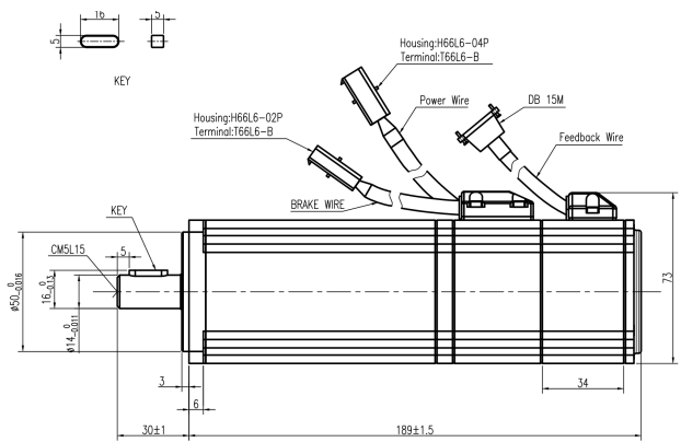
Mechanical View 9
