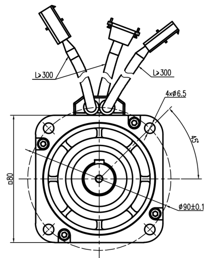
Mechanical View 9
